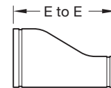
FIGURE 351 FABRICATED ECCENTRIC REDUCER (SEGMENT WELDED)
