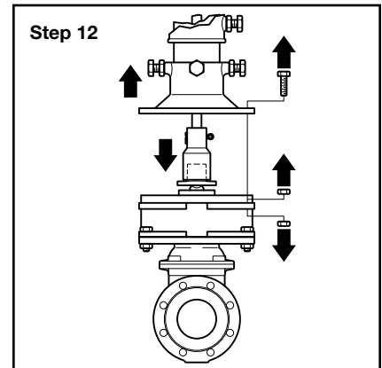
Step 12. Temporarily detach indicator from reducing gear and raise to gain access to reducing gear top cap. Engage connection tube coupling onto reducing gear top cap.
