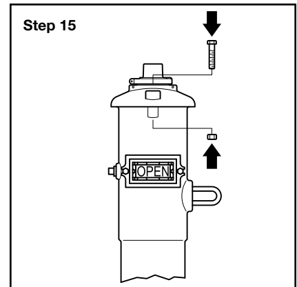
Step 15. Secure cap to body with bolts and nuts.
